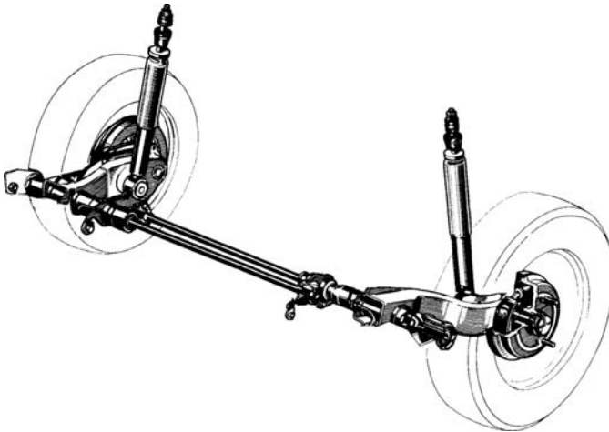
Figure 1.11.2 Plain trailing arms, 90° pivot axis, offset torsion-bar springs, unequal wheelbases (Renault).
