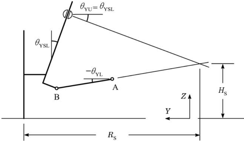
Figure 12.14.1 Strut-and-arm suspension, basic front-view geometry.
