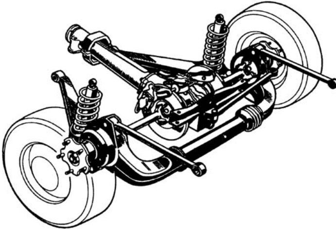
Figure 1.8.2 De Dion axle variation with sliding-tube variable track (1963 Rover).
