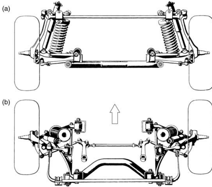
Figure 1.6.7 A passenger car double-wishbone system with a wide-base lower wishbone, and the upper wishbone partially defined by the anti-roll bar (Mercedes Benz).
