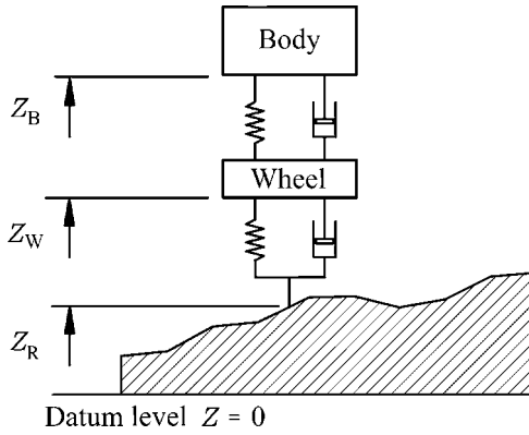
Figure 4.7.1 Body, wheel and road positions above the datum level.
