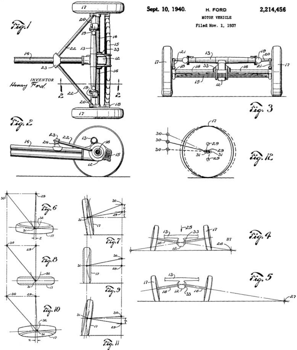
Figure 11.9.2 A swing axle with bump toe-out to compensate for side forces resulting from bump camber action (Ford, 1937).
