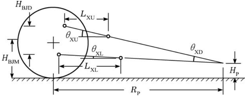
Figure 12.11.1 Equivalent two-dimensional side view of double transverse arms.
