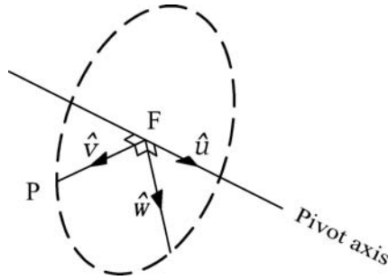
Figure 11.12.2 Generation of local coordinate system for rotation of a point about an axis by a specified angle.
