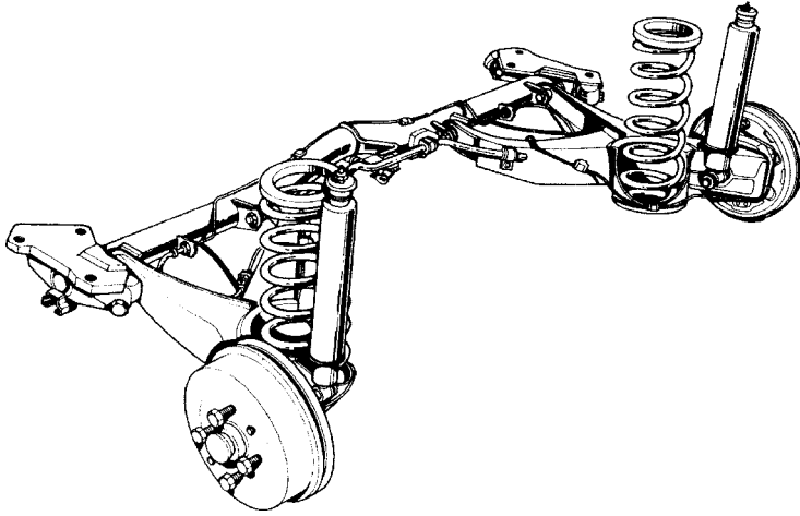
Figure 1.11.1 Plain trailing arms, 90° pivot axis, coil springs (Simca).
