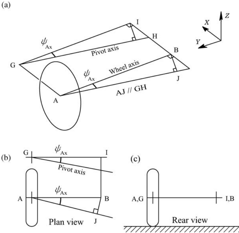
Figure 11.6.1 The basic semi-trailing arm, with pivot axis sweep angle \psi_{Ax} : (a) rear three-quarter view; (b) plan view; (c) rear view.
