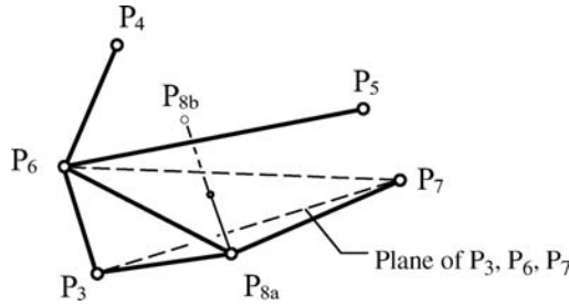
Figure 16.10.2 Two solutions by Points3S for the steering-arm end ball joint (track-rod outer end) in the case of double-transverse arms.
