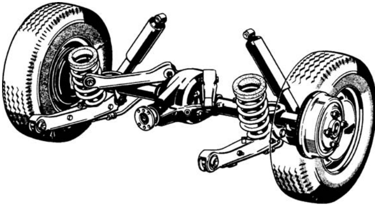
Figure 1.7.3 Widely-used design of four-link location axle (Ford).
