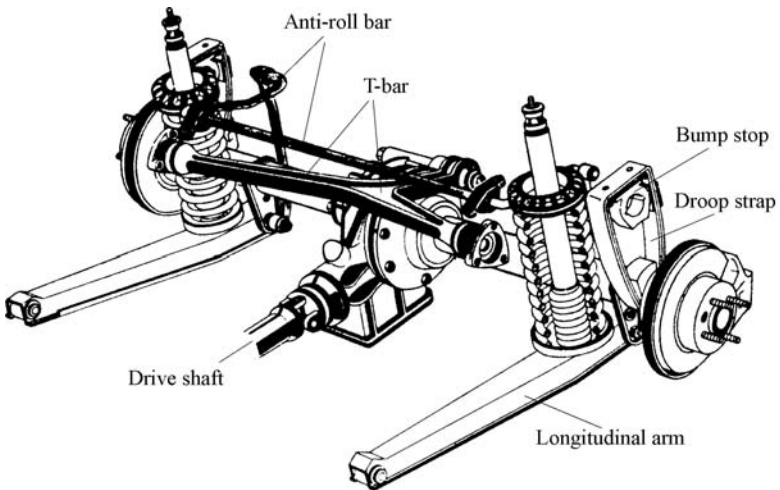
Figure 1.7.4 Alfa-Romeo T-bar upper lateral location.
