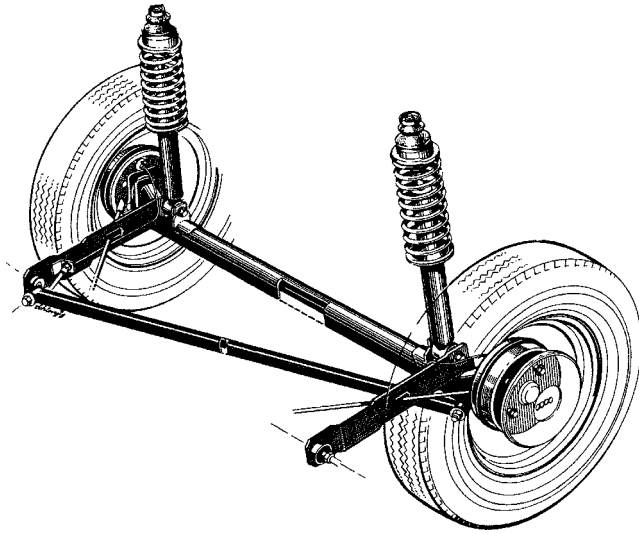
Figure 1.9.2 Undriven rigid axle with diagonal lateral location (Audi).
