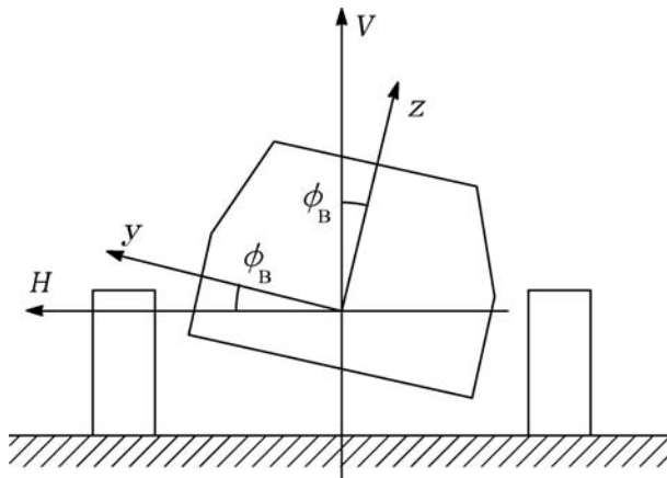
Figure 2.12.1 Accelerometer-carrying vehicle in rolled position.
