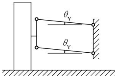
Figure 12.5.1 Angled parallel equal-length arms.
