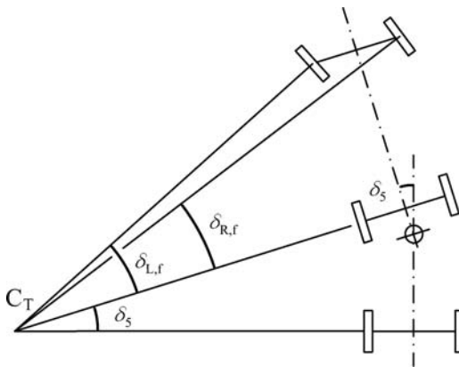
Figure 5.4.7 Kinematic turning of a car with a single-axle trailer.
