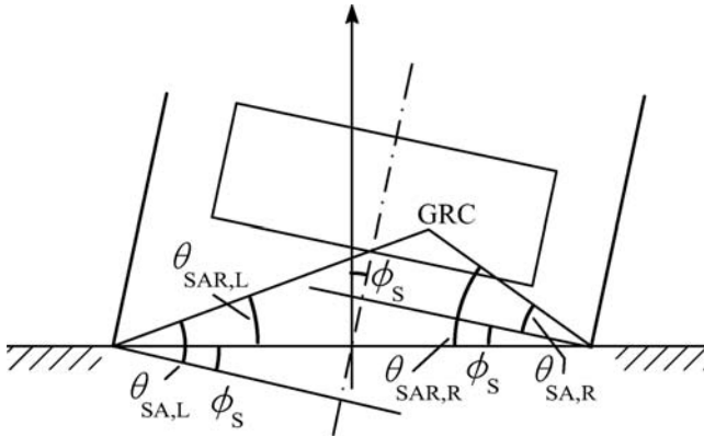
Figure 8.12.2 Rolled vehicle showing swing arm angles \theta_{SA} in vehicle coordinates and \theta_{SAR} in road coordinates.
