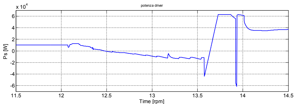
Fig. 3.60- EM generated power (negative)
