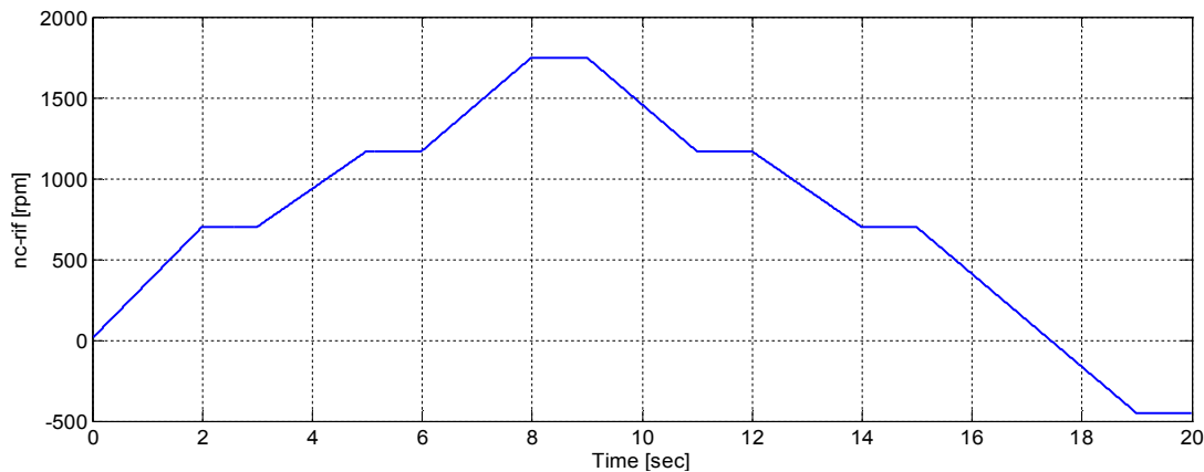
Fig. 3.40- Propeller speed profile
