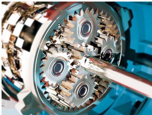
Fig. 1.1 – Planetary gear set layout
