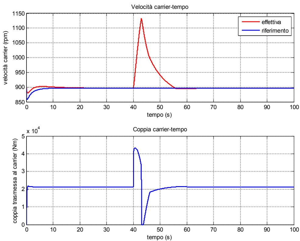
Fig. 4.20 – Simulation 2 – Carrier speed and torque
