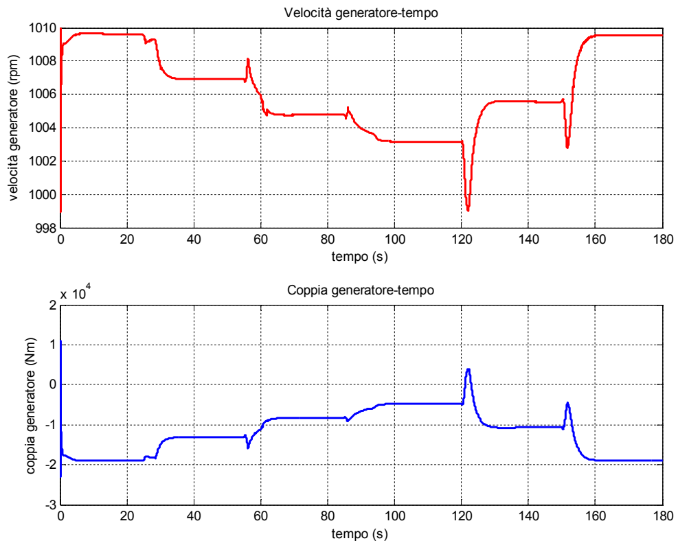
Fig. 4.15 – Simulation 1 – Generator speed and torque
