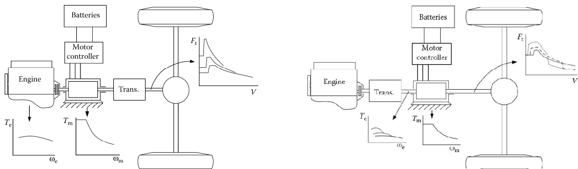
Fig. 1.9 –Parallel hybrid drivetrain- torque coupling – single shaft a. Before transmission b. After transmission
