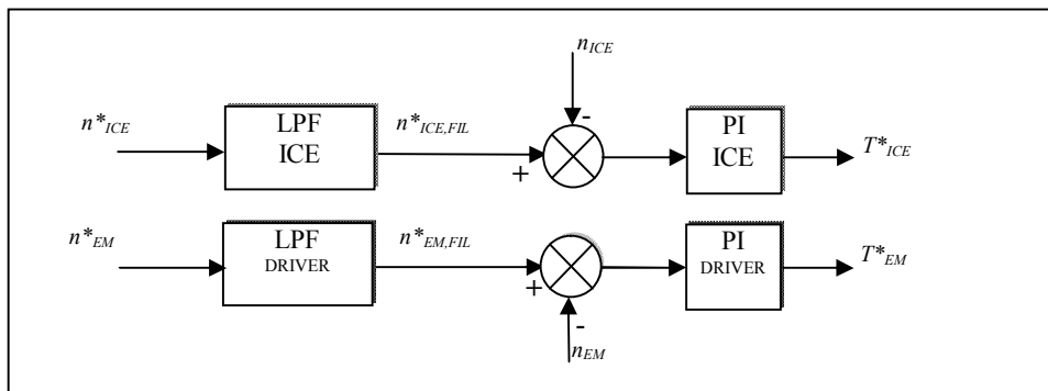
Fig. 3.24- Speed control loop
