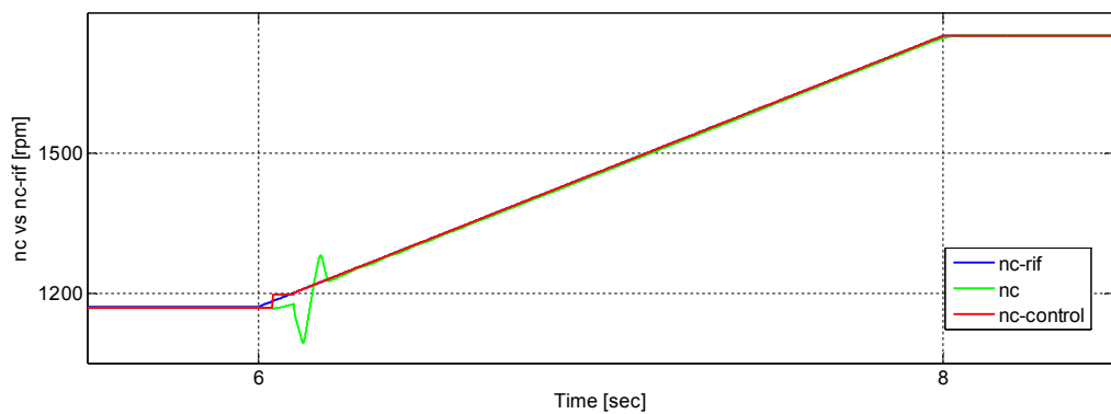
Fig. 3.52- Actual propeller speed nc (green), propeller speed setpoint nc_control (red)
