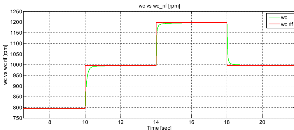
Fig. 3.36- Actual propeller speed wc (green), propeller speed setpoint wc\_rif (red)
