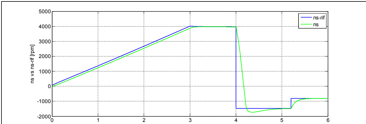
Fig. 3.67- Sun/EM actual speed (green), and its setpoint value (blue)
