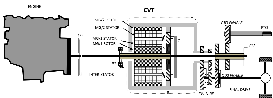
Fig. 2.1- Conceptual scheme of a power split drive for tractor propulsion
