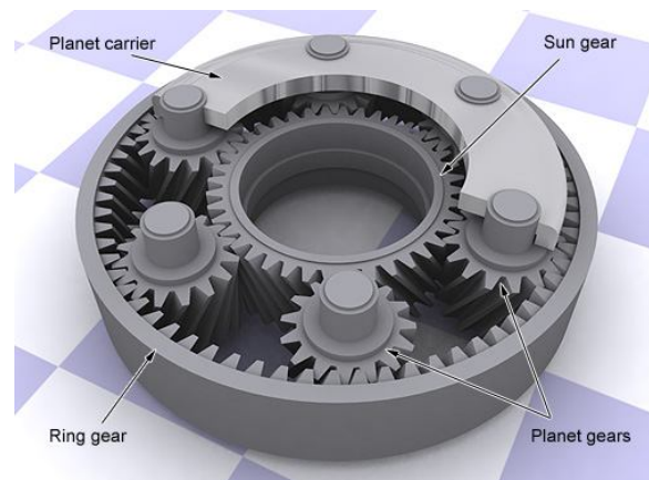
Fig. 1.1 – Planetary gear set layout
