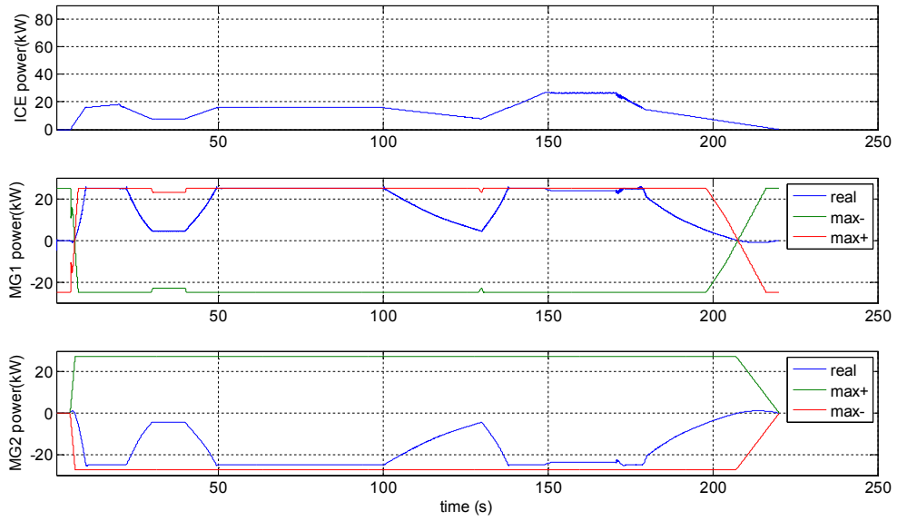
Fig. 2.20 – Simulation 1, Machines power
