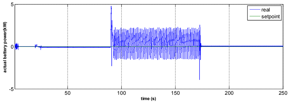
Fig. 2.33 – Simulation 3, Battery power
