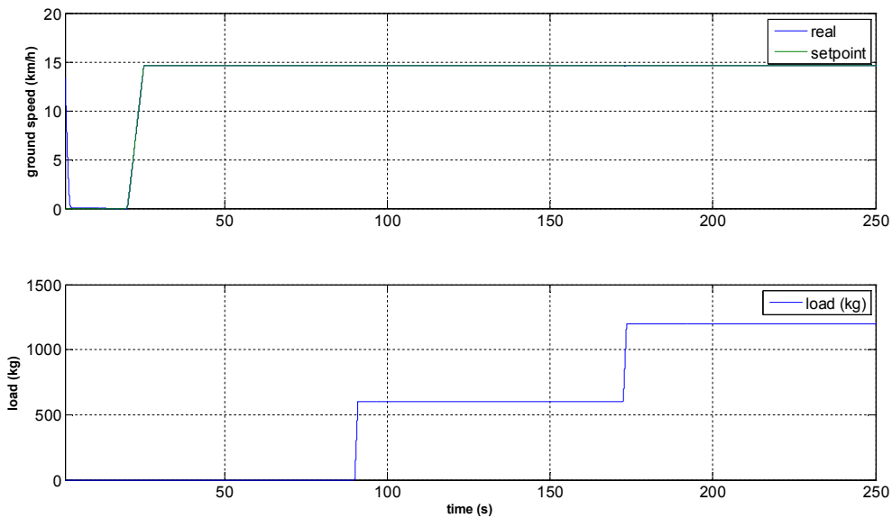
Fig. 2.28 – Simulation 3, ground speed and load
