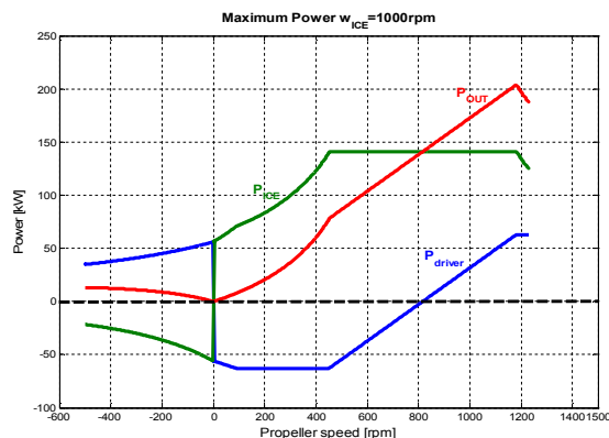
Fig. 3.13 - Maximum power in the three element of the transmission vs. propeller speed for \omega_{ICE}=1000 [rpm]. P_{ICE} : output power of the ICE; P_{driver} : output power of the driver; P_{out} : output power at the propeller shaft.
