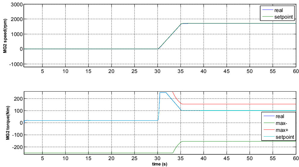
Fig. 2.43 – Simulation 5, MG/2 speed and torque
