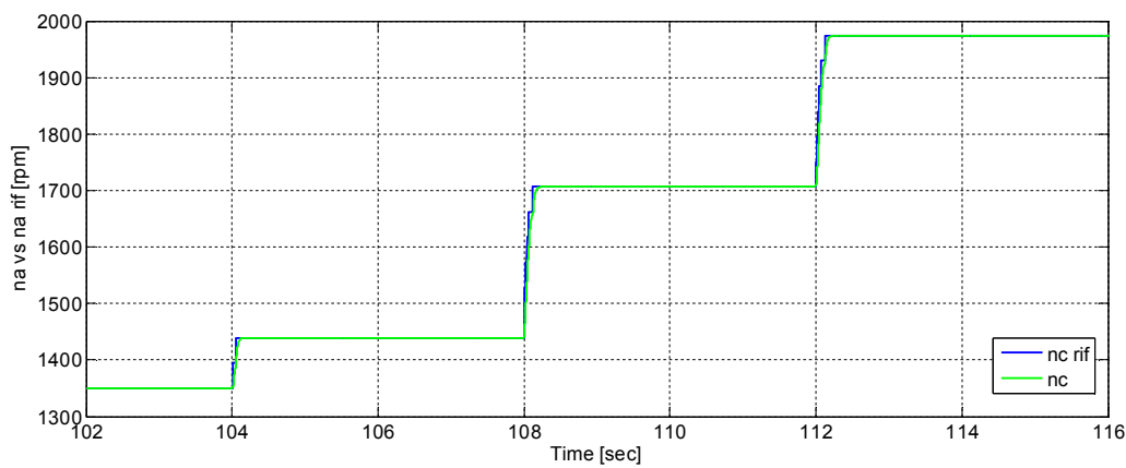
Fig. 3.33- Ring/ICE speed na (green), and its setpoint (blue)
