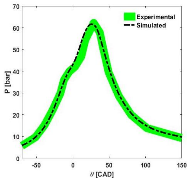
Figure 10: simulated in-cylinder pressure for gasoline-fueled EF7TC
