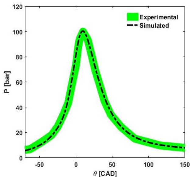
Figure 11: simulated in-cylinder pressure for CNG fueled EF7TC
