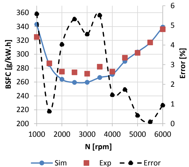
Figure 5: Simulated brake specific fuel consumption via experimental results for gasoline-fueled EF7NA
